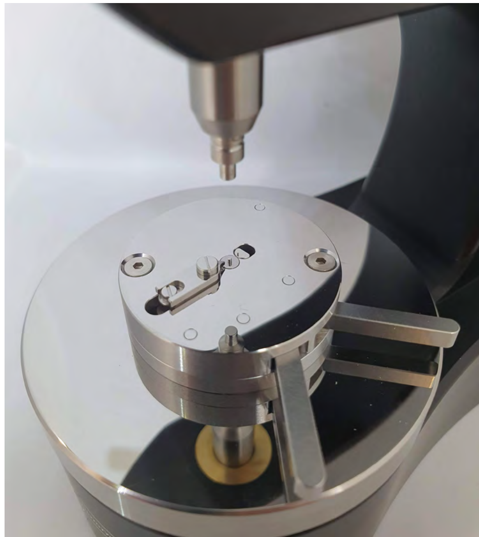
Developed and produced by Chatelain Prototypes: Assembly tool for the planetary gears in a watch mechanism.
